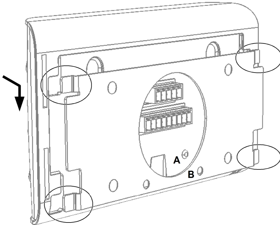
Figure 2: Fitting DRIFTER onto mounting bracket
